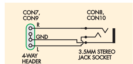
Fig.7: 4-way headers CON7 and CON9 are connected to the two 3.5mm stereo jack sockets. This makes it easy to connect to CD-ROM drive audio outputs via a standard stereo jack plug.
